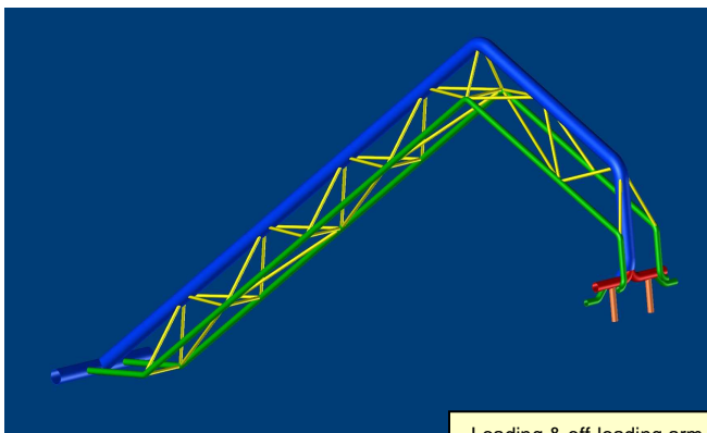
Loading & off-loading arm
